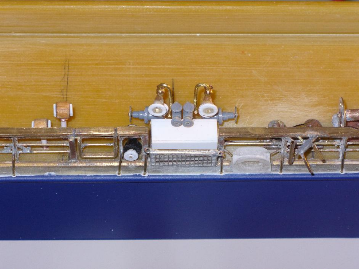
Almost the complete railing is soldered together in Brass material, the both gangways with their storings are done:
